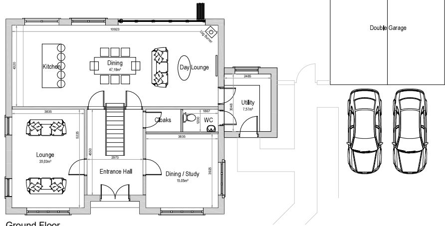
Ground Floor 247.80m 2 - Total Gross External Area - Excluding Garages
